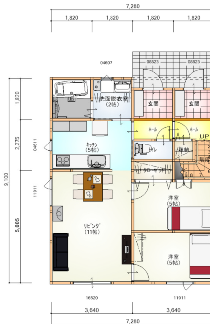
1st FLOOR
