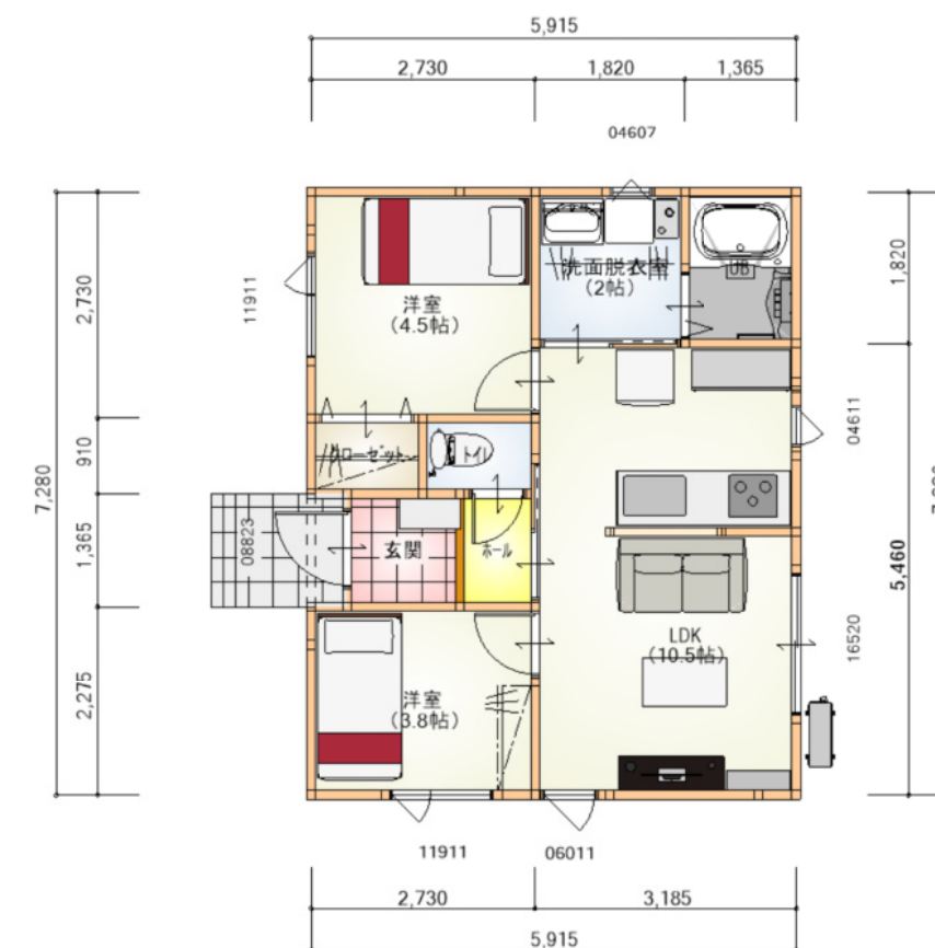
1st FLOOR
