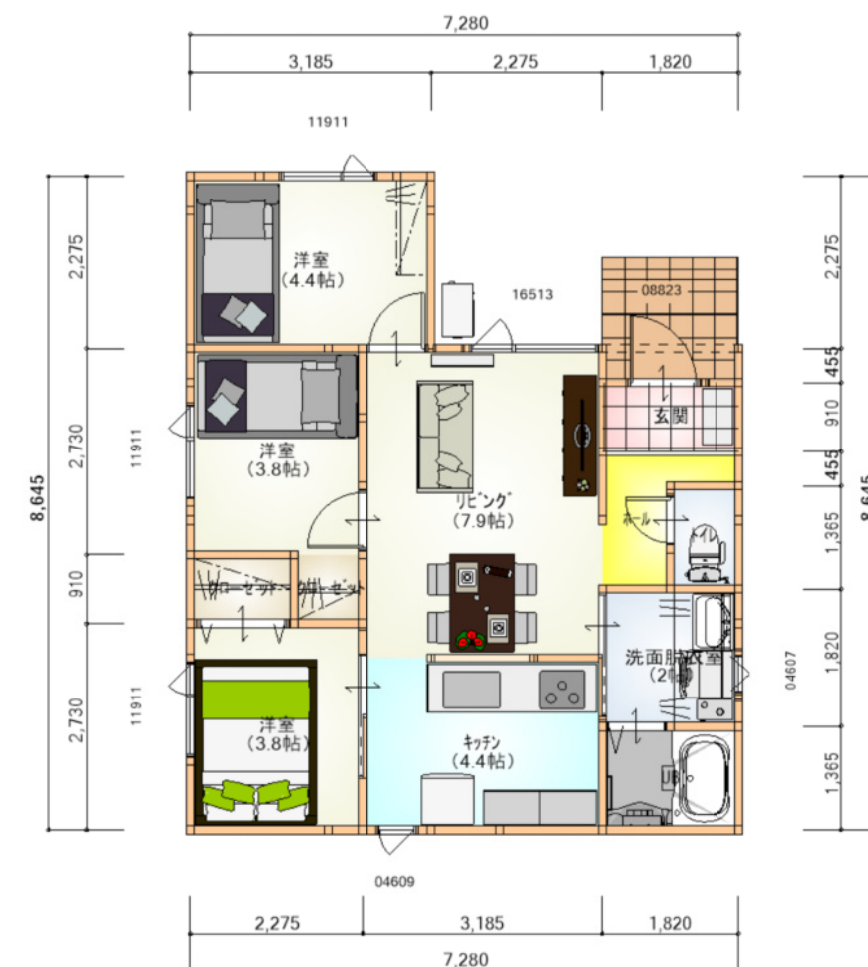
1st FLOOR
